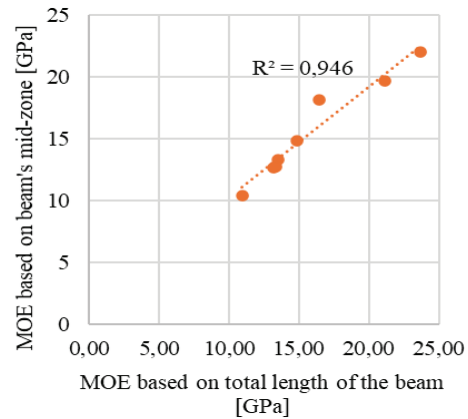
Figure 7 Correlation between the stiffness of the mid-zone and entire beam.
