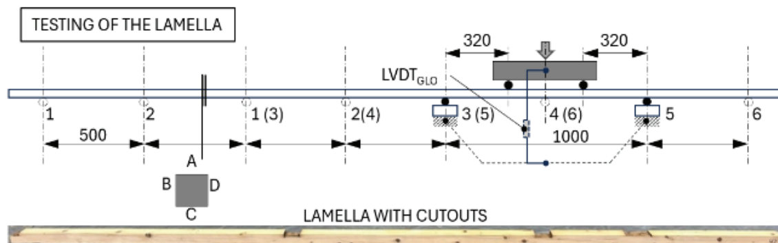
Figure 1 Marking of a test specimen and bending test setup according to the example in point 6.
