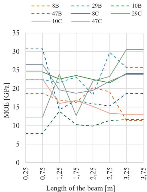
Figure 6 Stiffness values of the SBI-PUR beam lamellae.
