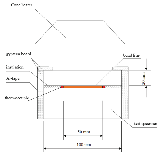
Figure 5 Test specimen setup under the cone heater.
