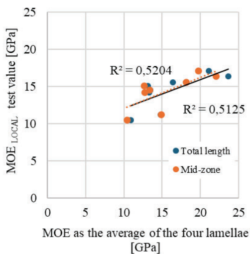
Figure 7 Correlation between the average stiffness of individual lamellae and the measured local MoE.
