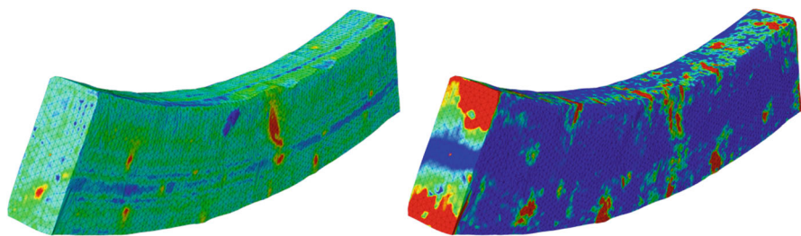
Fig. 7 FE model for a partial section of the beam, density field (left) and corresponding absolute transverse stress field (right)
