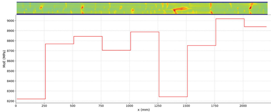
Fig. 8 Bending stiffness profiles for the evaluated sections of the studied beam. The average density along the thickness direction is plotted on top, and red colours indicate higher and blue lower values
